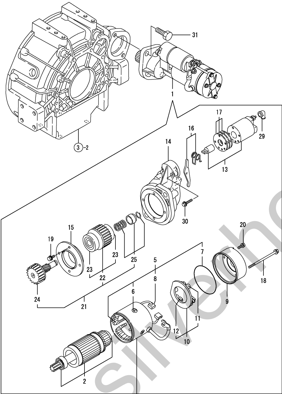
Fig.16. STARTING MOTOR
