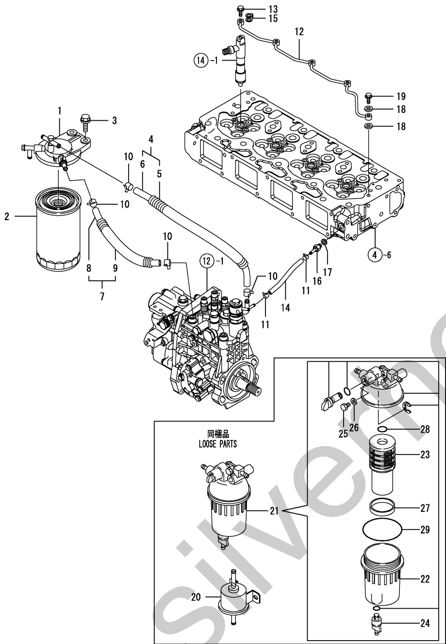
Fig.15. FUEL LINE
